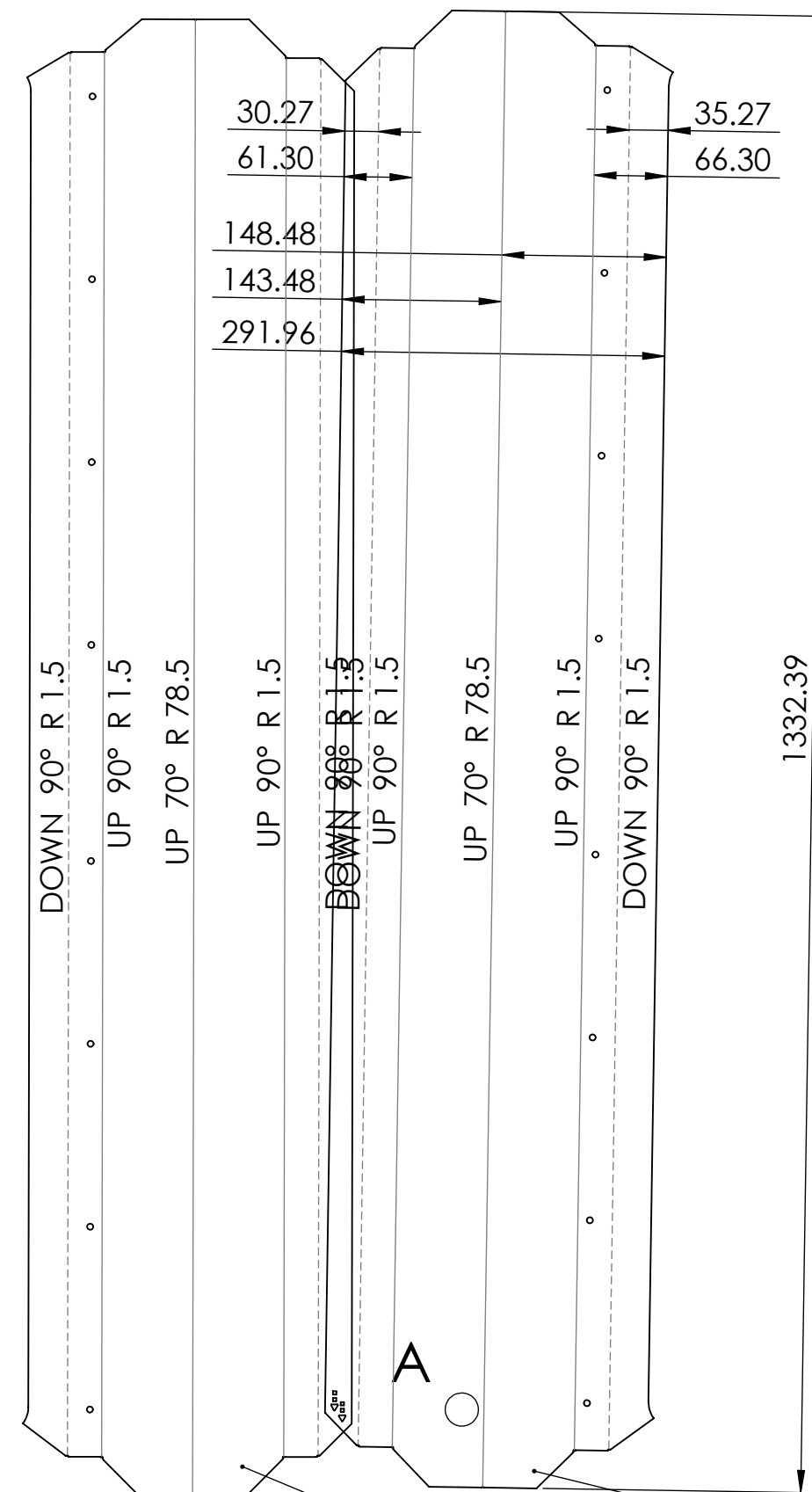
TOD6-09 v1.2L, SM-FLAT-PATTERN TOD6-09 v1.2R, SM-FLAT-PATTERN
